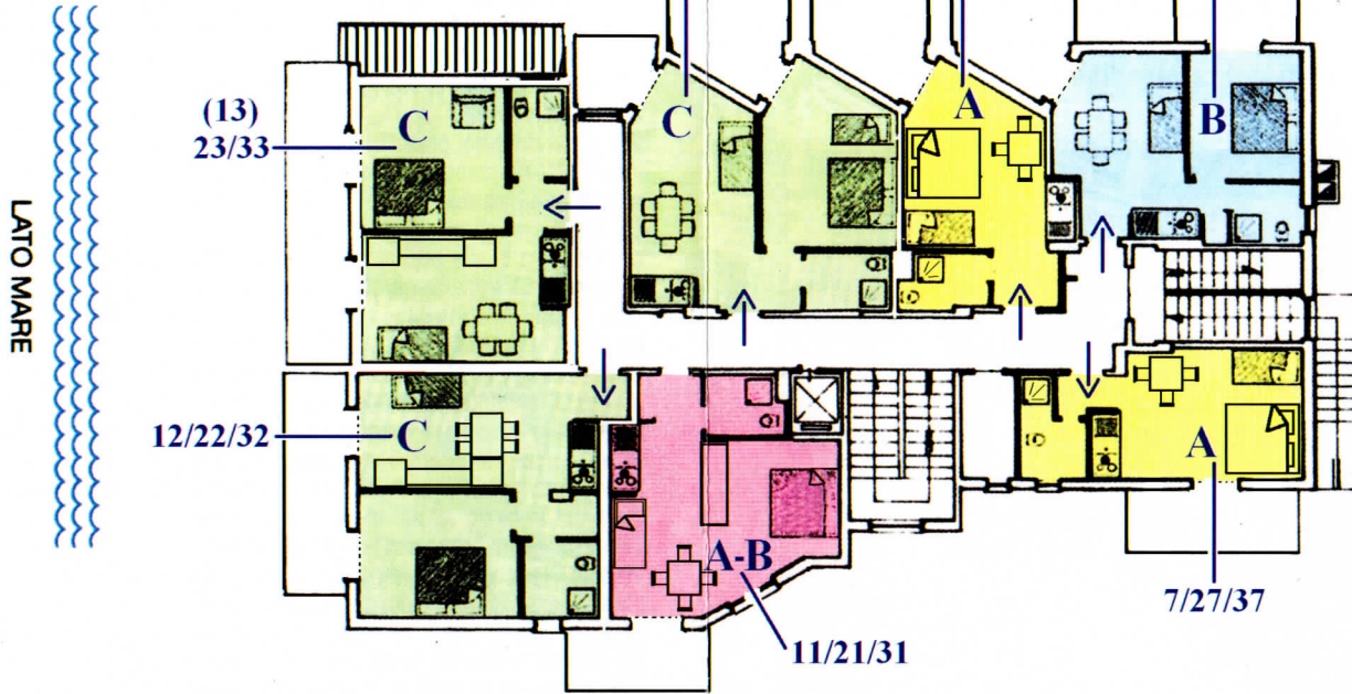
PIANTA 1°/2°/3° PIANO
